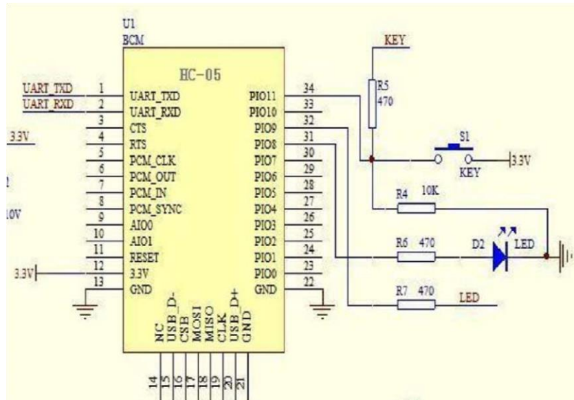
Figure 7 Application 1
