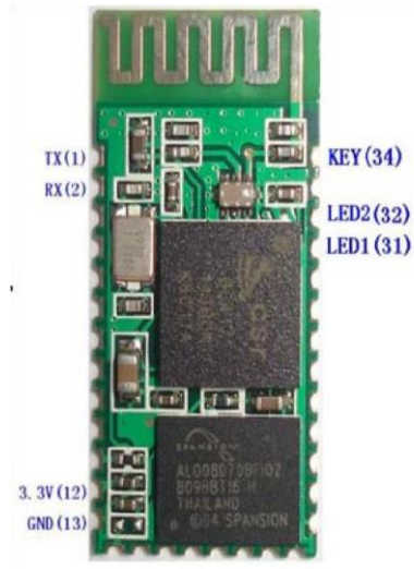
Figure 2 HC-05
