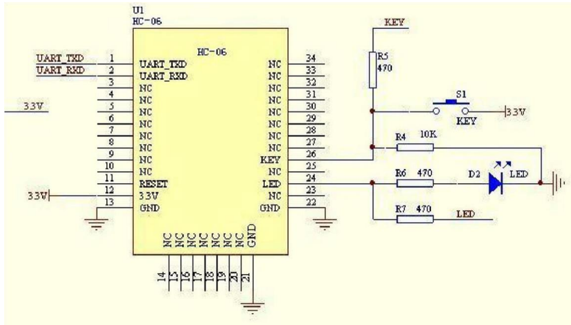
Figure 5 The circuit 1
