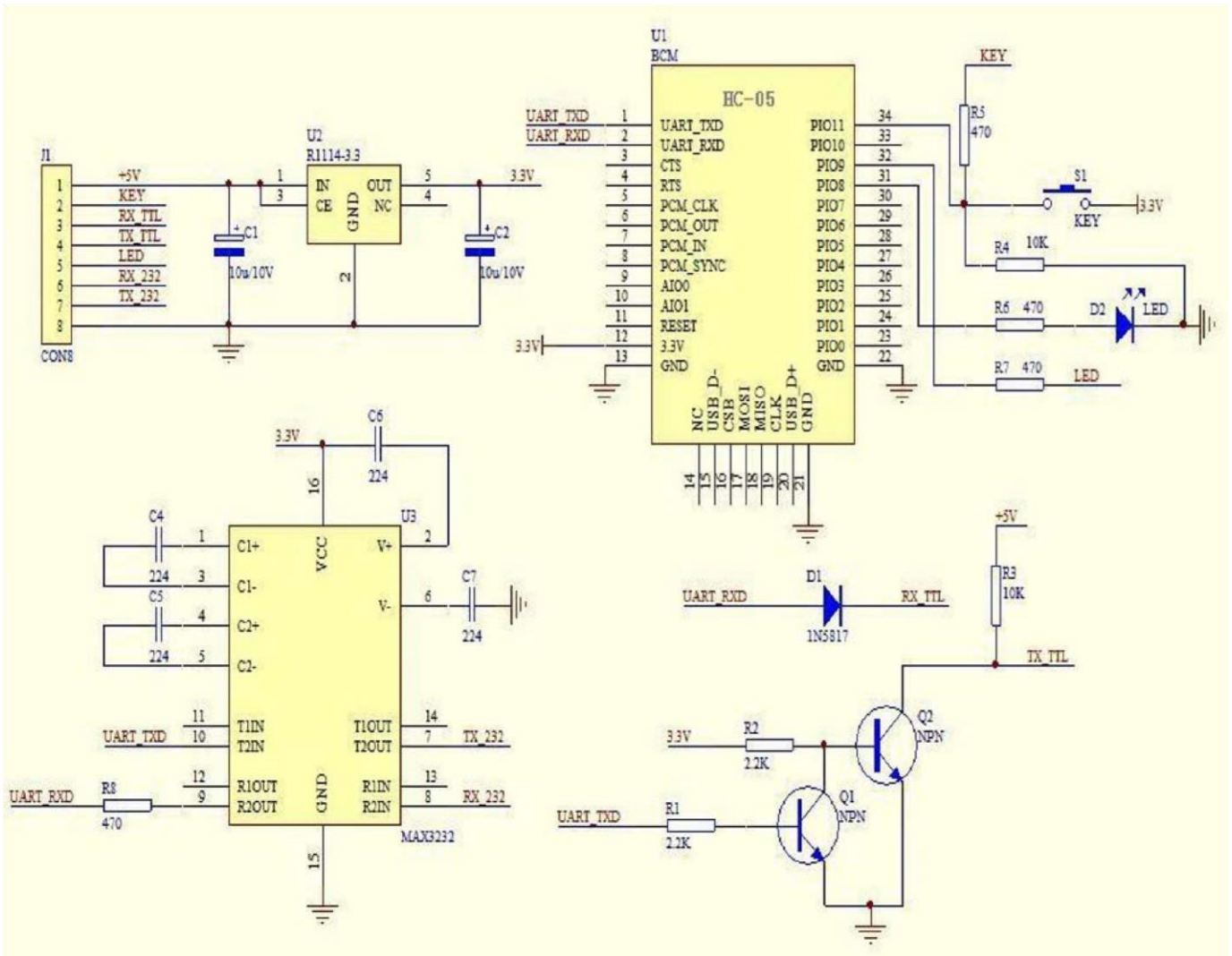
Figure 8 Application circuit 2
